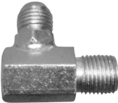
COTOVELO 90° MO UNF X MJ UNF
